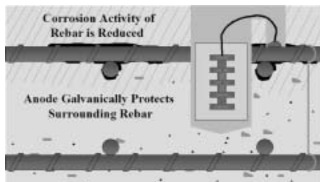
Fig. 3—Chloride-accelerated corrosion.
