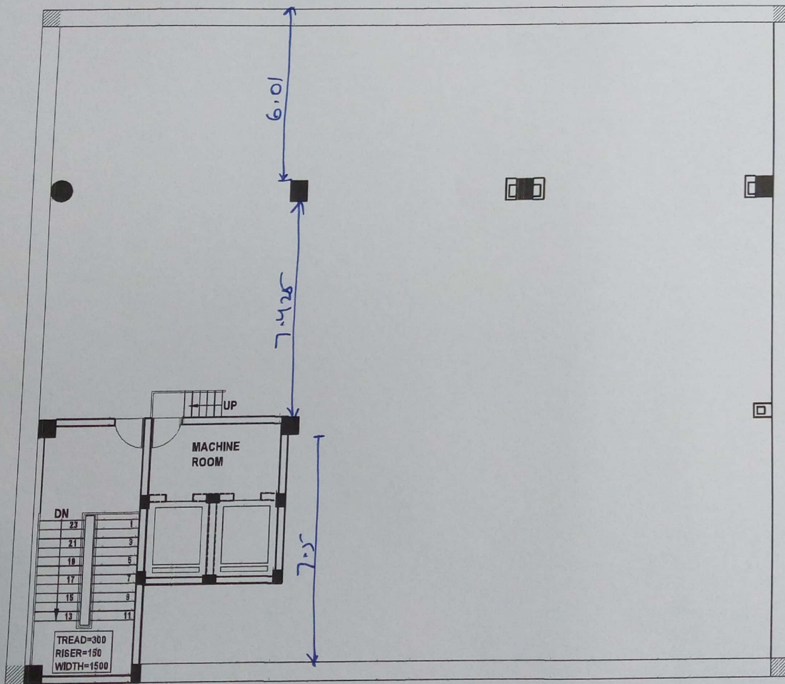
TERRACE PLAN
